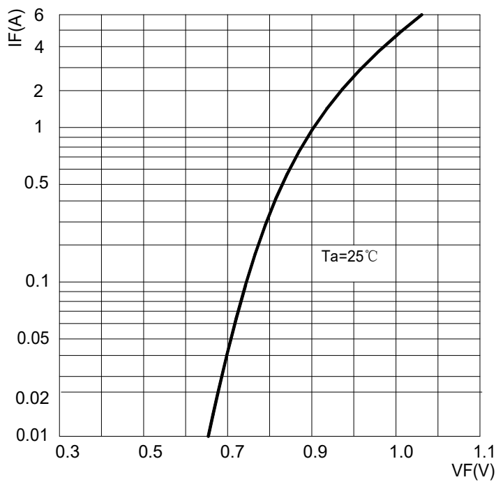
FIG.3: Forward Voltage
