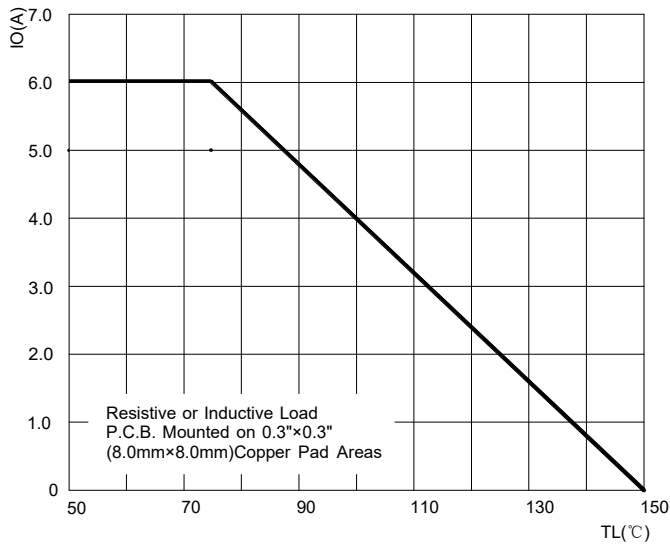
FIG.1: Io-TL Curve
